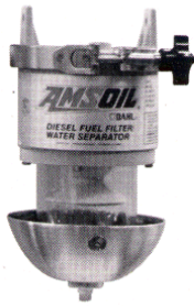
ADF11 Diesel Fuel Filter/Water Separator U.L. Listed and U.S. Coast Guard Accepted for Marine Applications
