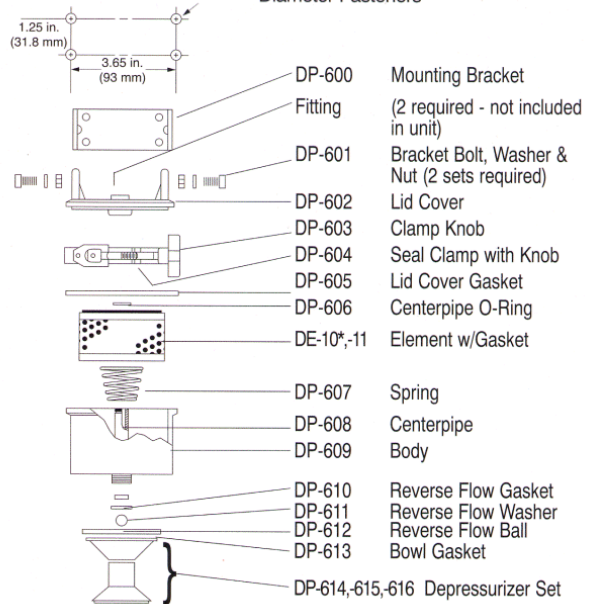
ADF11 Diesel Fuel Filter/Water Separator U.L. Listed and U.S. Coast Guard Accepted for Marine Applications
